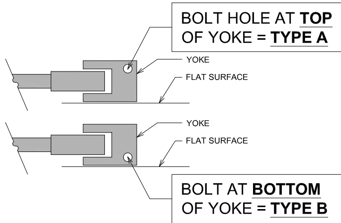
2 SIDE VIEW OF STEERING SHAFT YOKE SK1 SCALE: NTS
